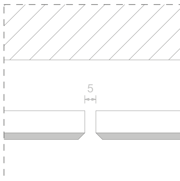
04 Fibrocemento - Pannello contiguo FBC Butt Joint
